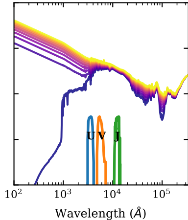
Dusty
