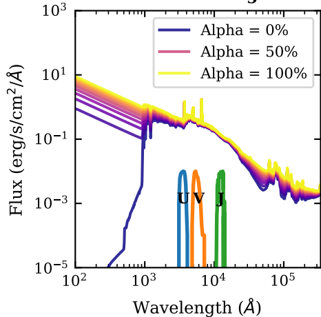
Star-forming
